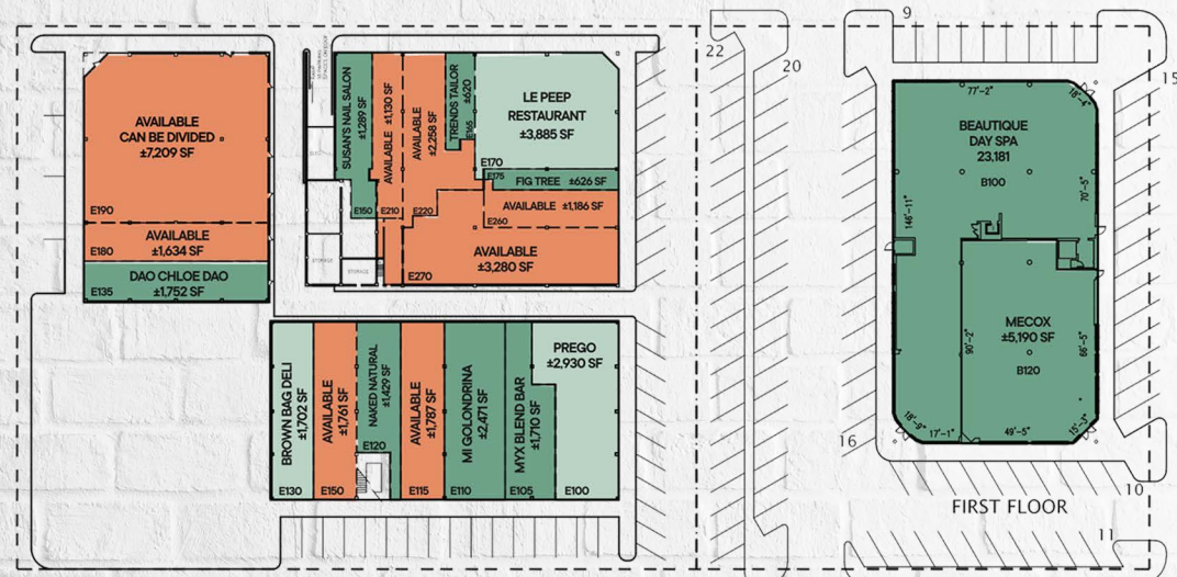
FLOOR PLAN - BUILDING B - LEVEL 1 SCALE: 1" = 50'
